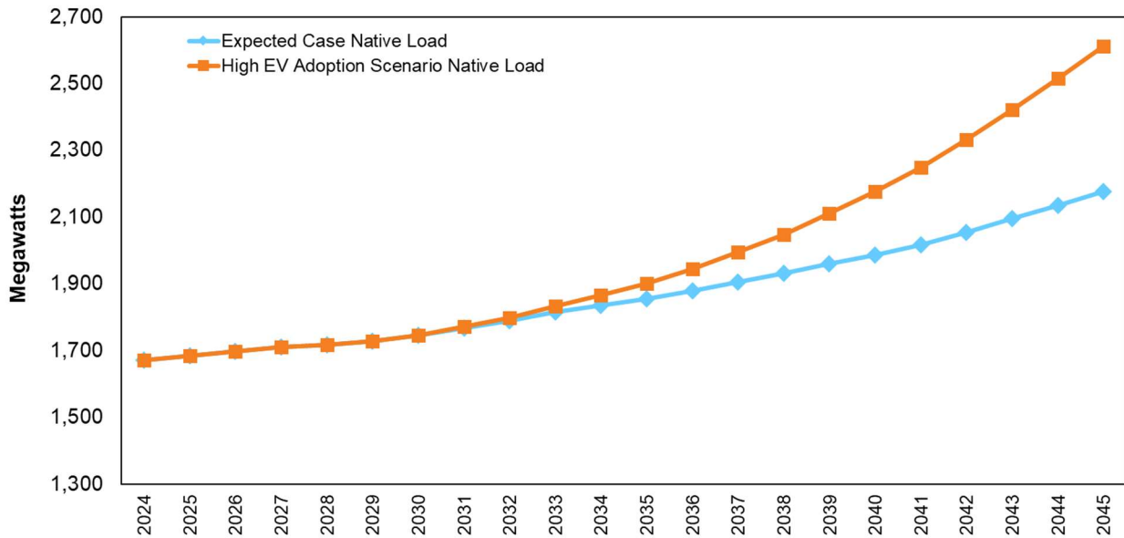
Figure 2.28: High EV Adoption – Summer Peak Impact
