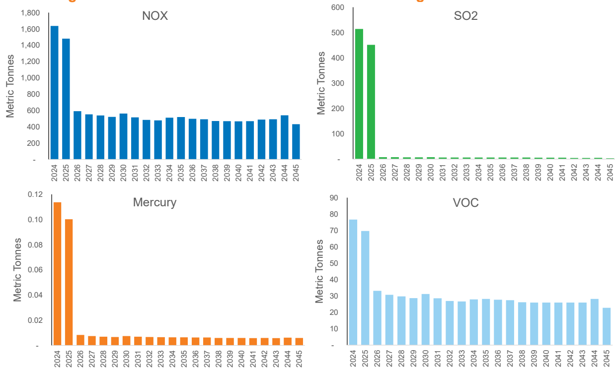
Figure 9.12: Avista Owned and Controlled Generating Plant Air Emissions
