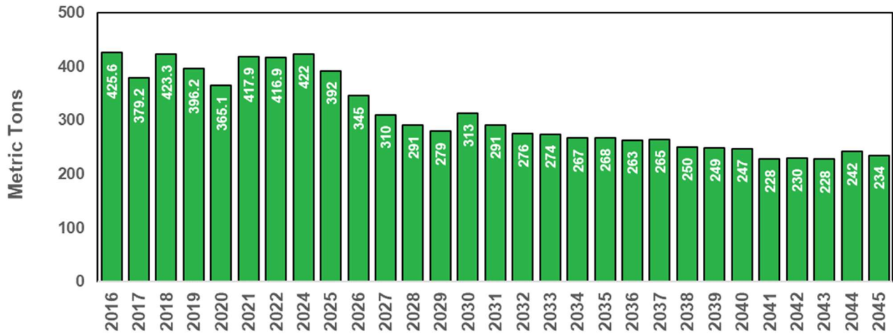
Figure 11.15: Avista's Washington State Facility's NO x Emissions
